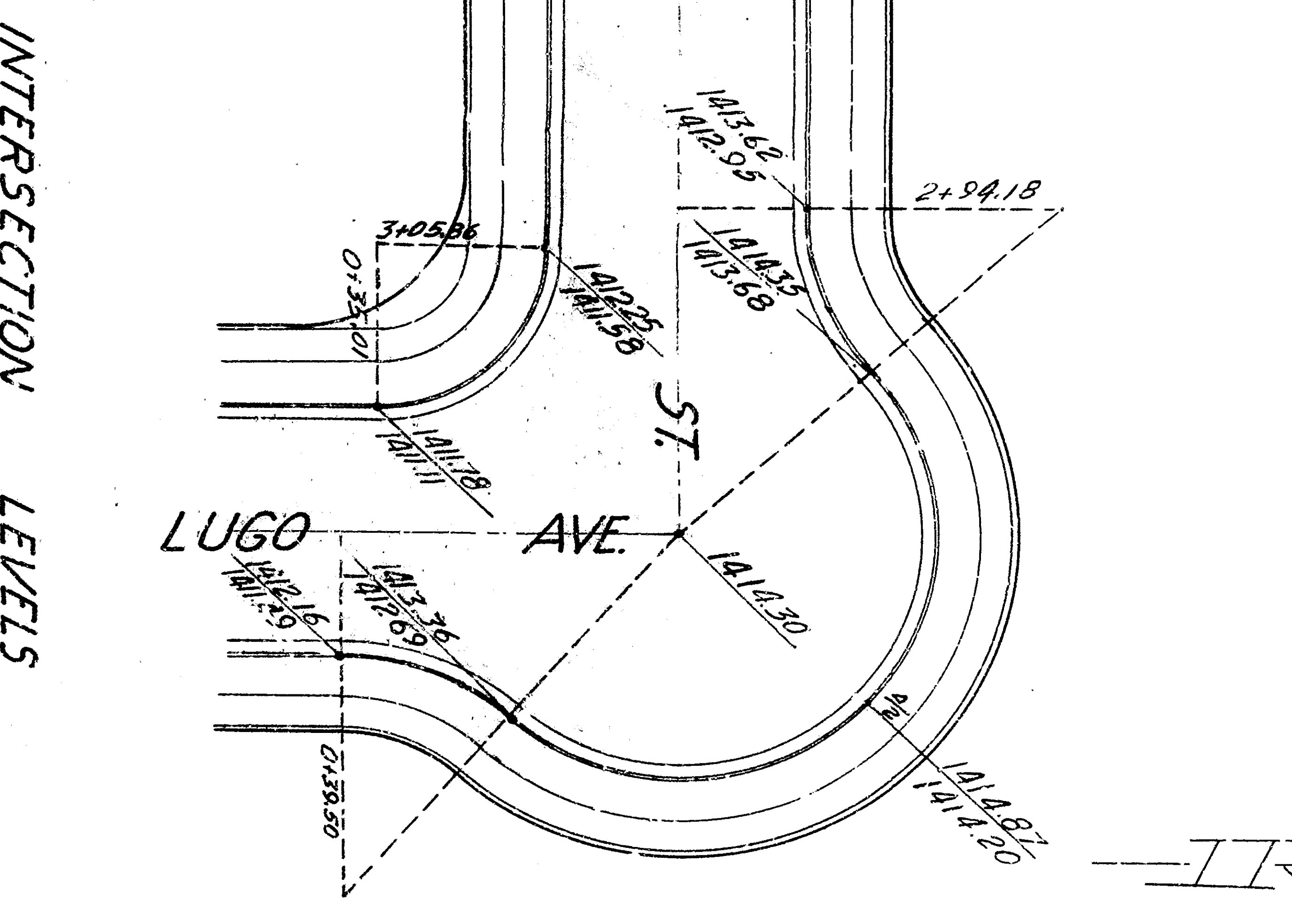
INTERSECTION LEVELS SCALE: 1"=20'
